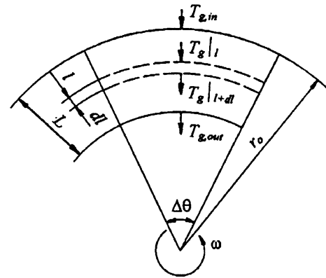
Fig. 2. A differential section in a centrifugal fluidized bed.
